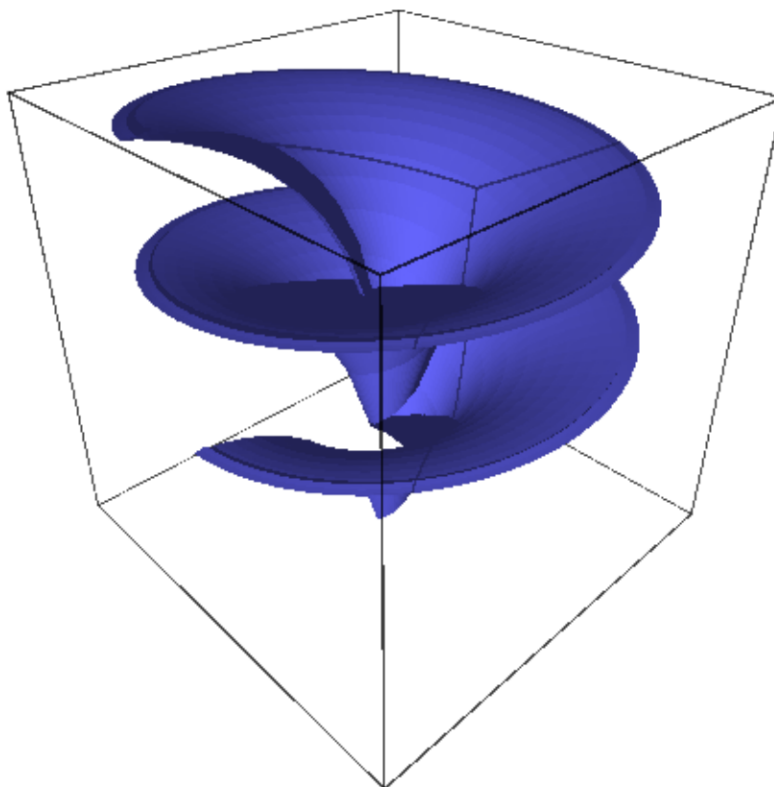
The Hesseberg surface:
